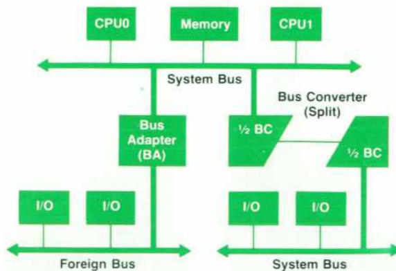
Fig. 3. Large HP Precision system configuration.
