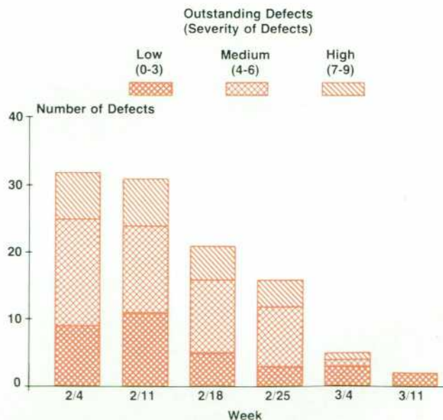
Fig. 4. Defect backlog plot.
