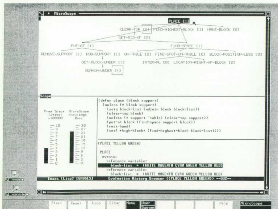
Fig. 5. A screen from MicroScope, a knowledge-based program analysis tool, showing a call graph monitoring program execution, the source code of the highlighted module, evaluation history browser, and system resource monitors.
