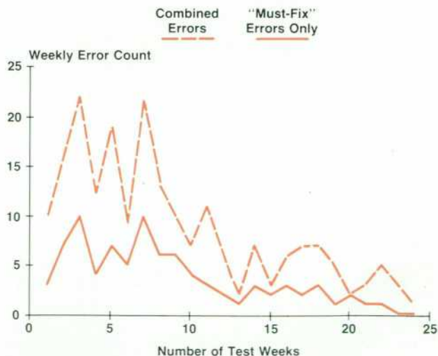
Fig. 5. Rate of error detection during the software testing phase.
