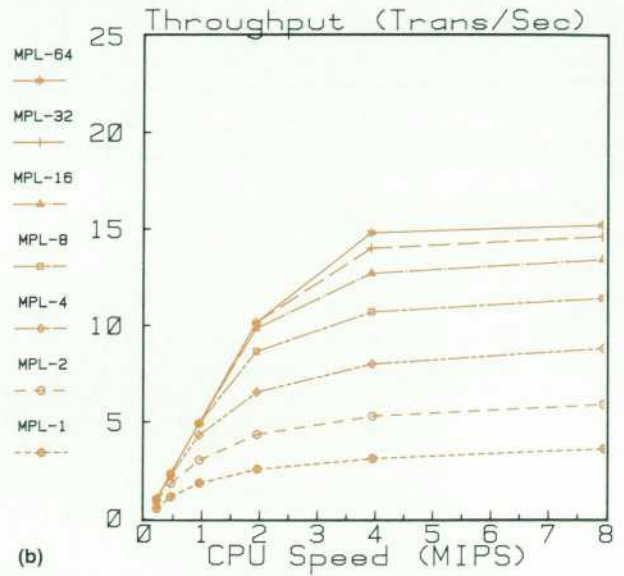
No Disc Caching with 4 10-ms Discs
