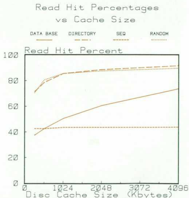
Fig. 13. Potential benefit of disc caching for the HP 3000 family is shown by this graph of read hit rates that can be achieved by various access methods as a function of cache capacity.
