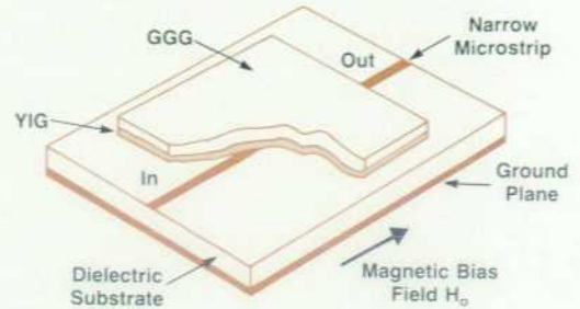
Fig. 14. Basic structure of an MSW signal-to-noise enhancer (Adam, et al 10 ).
