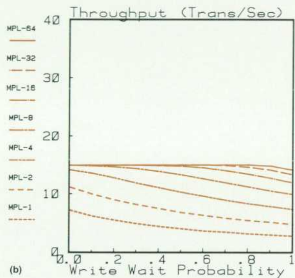
Write Wait Dependency with File Mapping: 3-MIPS CPU with 25-ms Discs and Read Hit Prob. = .85
