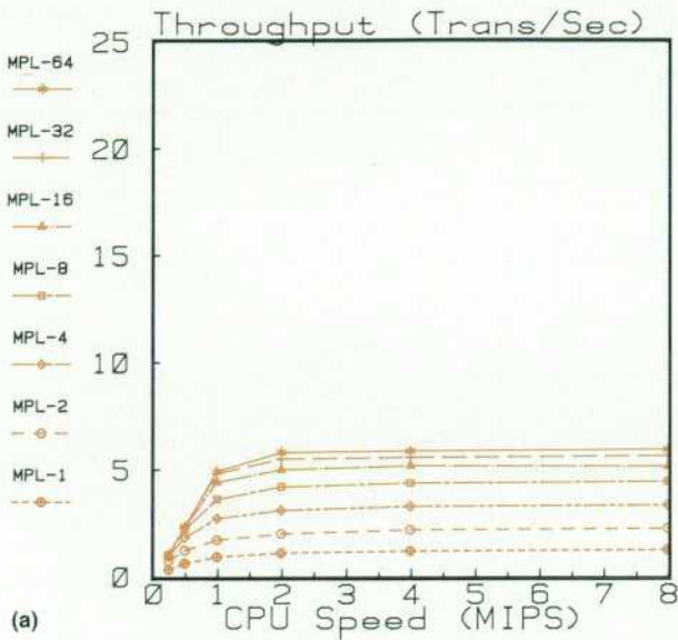
No Disc Caching with 4 25-ms Discs
