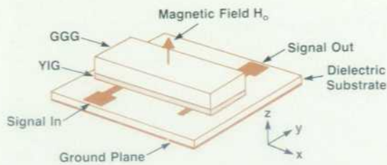
Fig. 4. Basic configuration of a magnetostatic-wave delay line.
