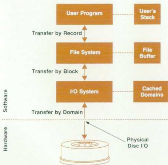
Fig. 14. Explicit internal disc cache interfaces in the breadboard MPE operating system kernel developed for this study.
