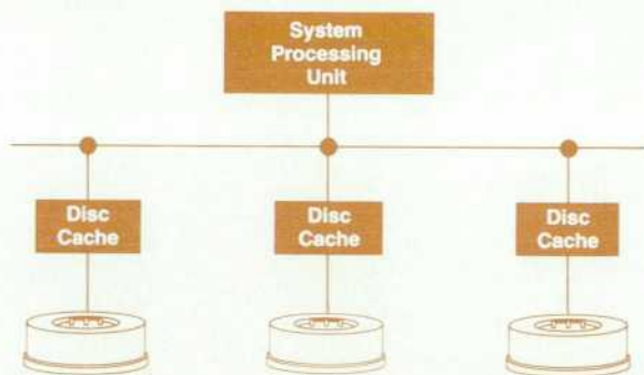
Fig. 3. External disc caching using a local buffer for each disc.
