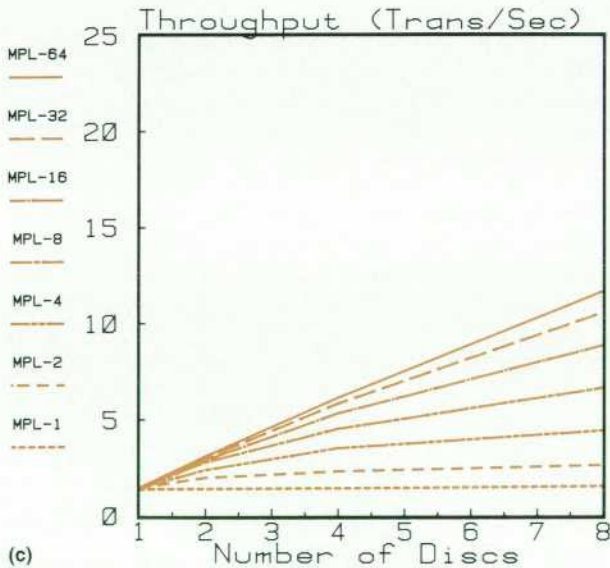
Fig. 2. Performance of systems using conventional memory hierarchies without disc caching. Transaction throughput is shown as a function of effective multiprogramming level (MPL), the number of processes that can be concurrently executed. The top graphs show throughput versus CPU speed for a fixed number of discs. The bottom graphs show throughput versus number of discs for a fixed CPU speed.
