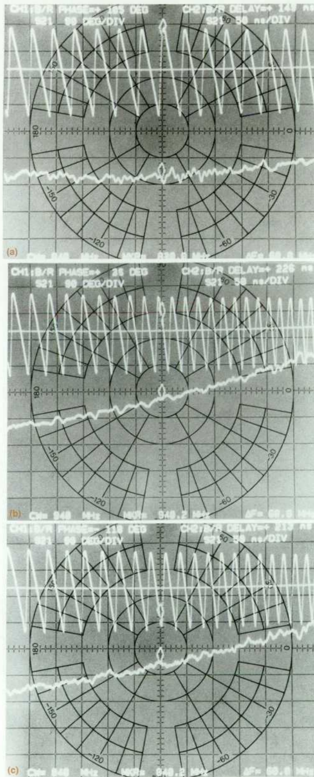
Fig. 6. Group delay (lower trace, 50 ns/div) and phase (upper trace, 90 degrees/div) characteristics for a tunable magnetostatic-wave delay line versus frequency (10 MHz/div). (a) Center frequency = 840 MHz, H_0 = 85 oersteds, relatively constant delay. (b) Center frequency = 940 MHz, H_0 = 85 oersteds, dispersive delay. (c) Characteristics of (b) tuned for center frequency of (a) by decreasing H_0 to 70 oersteds.
