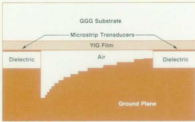
Fig. 7. Cross section of an MSW delay line using continuously varying YIG-film-to-ground-plane spacing 6 to linearize the dispersion characteristic (see Fig. 8).
