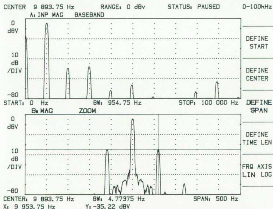
Fig. 3. Simultaneous display of baseband (upper trace) and zoom (lower trace) spectra can be selected for the HP 3561A's CRT.
