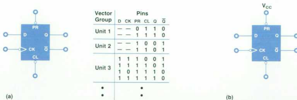
Fig. 5. (a) D-type flip-flop and library test sequence. (b) Use of flip-flop on board under test. For this topology, the library test is modified by removing test vector unit one.
