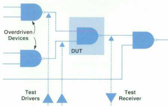
Fig. 1. In-circuit test connections to a NAND gate.
