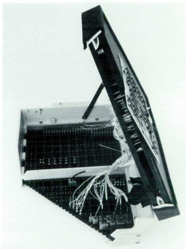
Fig. 5. Cutaway view of test fixture. Contact to the board under test is made by using vacuum to pull the board down onto a configuration of spring-loaded pins (bed of nails). The HP 3065 tells the user how to wire these pins to the test fixture.
