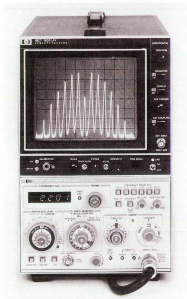
Fig. 1. The Model 8559A Spectrum Analyzer, shown here mounted in a Model 182T large-screen display, covers a frequency range of 0.01 to 21 GHz with accuracy and sensitivity characteristic of a lab-grade analyzer. Its size and weight make it suitable for field use.
