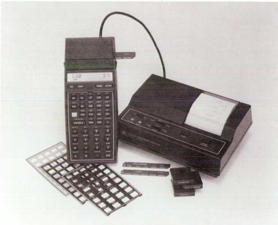
Fig. 1. The new HP-41C Calculator can be expanded like a computer system to include add-on semiconductor memory, mass memory, and hard-copy output. Here the HP-41C is shown with add-on memory modules and its optional magnetic card reader and thermal printer.
