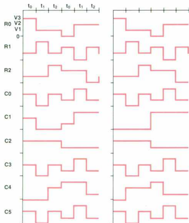
Fig. 5. Display drive waveforms to produce letters H and P. Voltages V1, V2, V3 are 1.1V, 2.2V, and 3.3V. An LCD segment is on if the rms difference between the row and column voltages applied to it is 2.1V. The segment is off if this rms difference is 1.1V.
