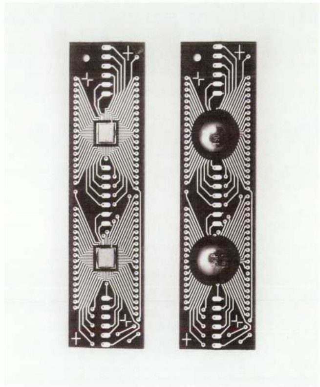
Fig. 4. Display driver module contains two chips, each measuring 4.17 by 3.63 mm. There are 54 bonds per chip, 14 connections to the HP-41C, and 72 connections to the liquid crystal display. Reflow-soldered contact tabs connect to the mainframe and flexible conductive strips connect to the LCD. The substrate measures 67.31 x 16.51 x 0.79 mm.
