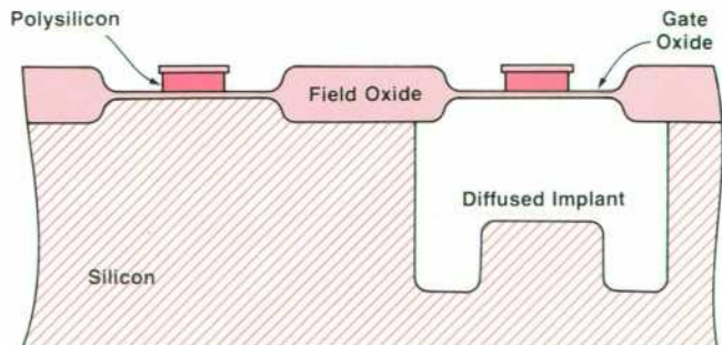
Fig. 2. Polysilicon gate definition is next. Then the gate oxide is etched away and the P+ and N+ source and drain diffusions are done (see Fig. 3).
