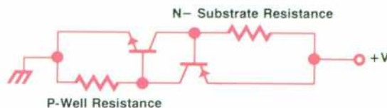
(b) Equivalent circuit of PNPN parasitic device
