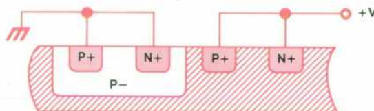
(a) CMOS cross-section
