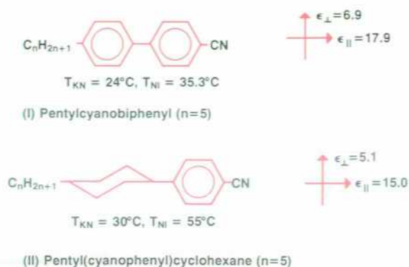
Fig. 2. Structures and properties of two commercially available nematic liquid crystal materials. The HP-41C display uses four compounds similar to type I.
