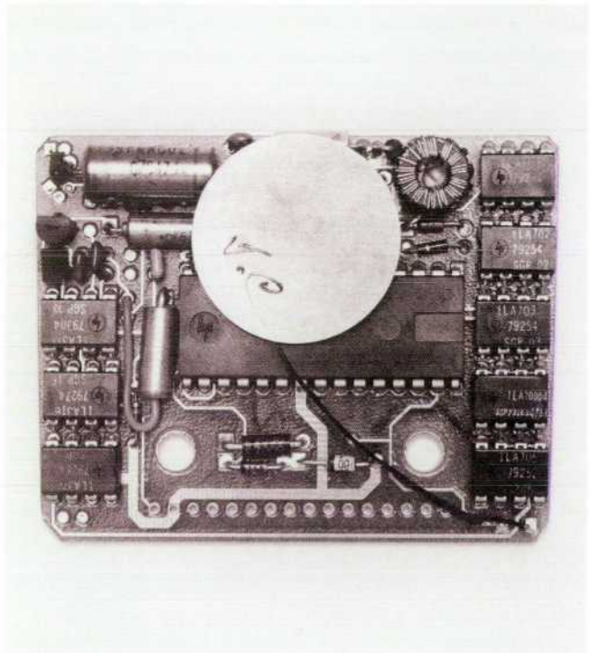
Fig. 2. HP-41C logic board.
