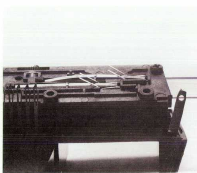
Fig. 2. A new card-detection switch design eliminates critical adjustments.
