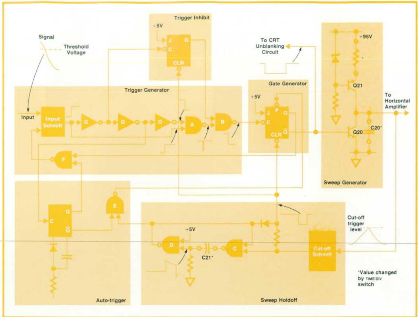
Fig. 9. Trigger and sweep generating circuit uses two holdoffs to prevent erratic sweeps (see text).
