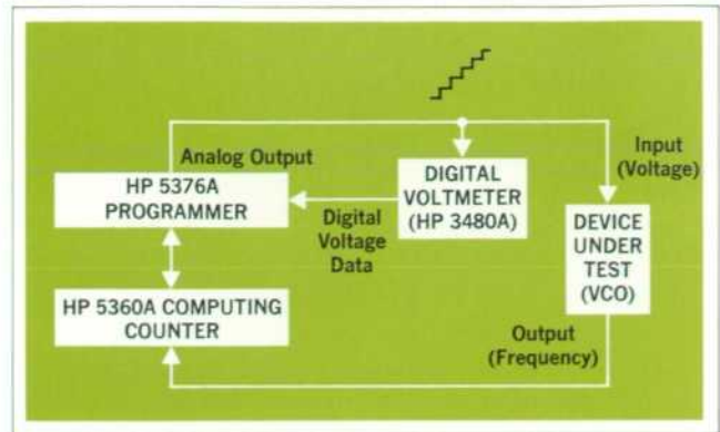
Fig. 7. Computing-counter system to measure integral nonlinearity.
