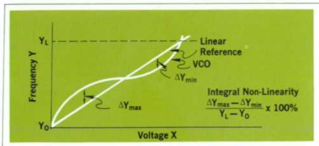
Fig. 6. Integral nonlinearity of a voltage-controlled oscillator.
