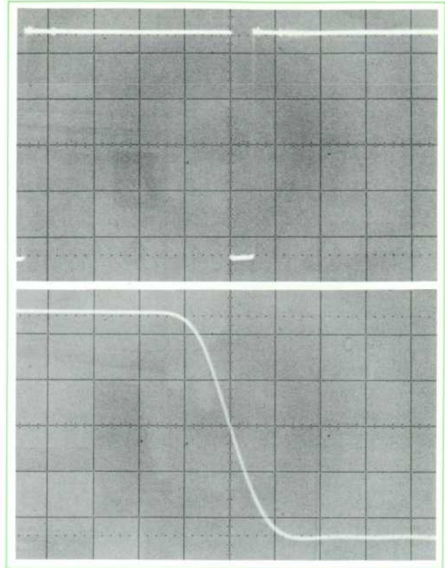
Fig. 6. Calibrating waveform. Sweep time in upper photo is 0.2 \mu\text{s}/\text{cm} ; in lower photo it is 1 ns/cm. Fast risetime provides check on scope's frequency response. Clean waveform is also useful as test signal for external equipment.
