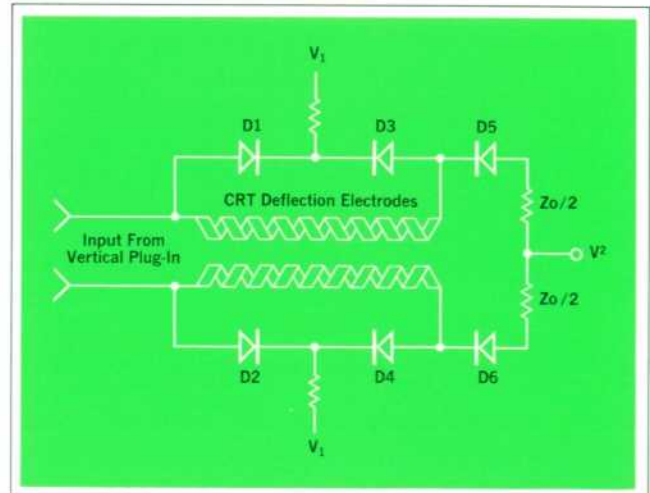
Fig. 7. Diodes switch CRT deflection electrodes to match amplifier source impedance. When Model 1830A plug-in is used, voltages V_1 and V_2 are both higher than deflection electrode voltage, connecting electrodes to terminating impedance Z_o . With other plug-ins, V_1 and V_2 are lower than electrode voltage, shorting electrodes end to end and disconnecting Z_o .
