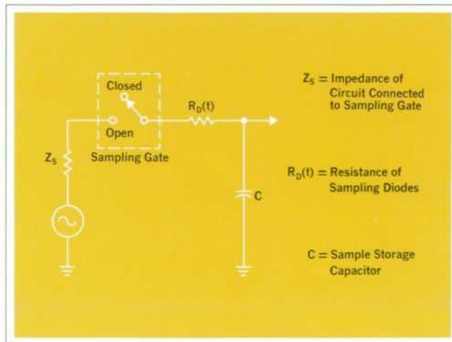
Fig. 14. Simplified diagram of sampling circuit.
