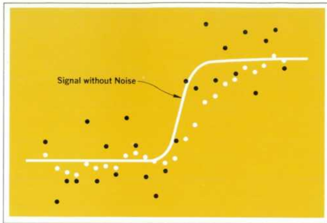
Fig. 11. Display of voltage step by sampling scope set for 100% sampling efficiency (black dots) and for 25% sampling efficiency (white dots). Note smoothing of response with reduced sampling efficiency, and consequent loss of risetime. (Horizontal dot spacing is exaggerated for purposes of illustration.)
