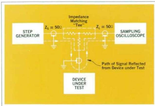
Fig. 2. Time domain reflectometer using ordinary lab instruments.
