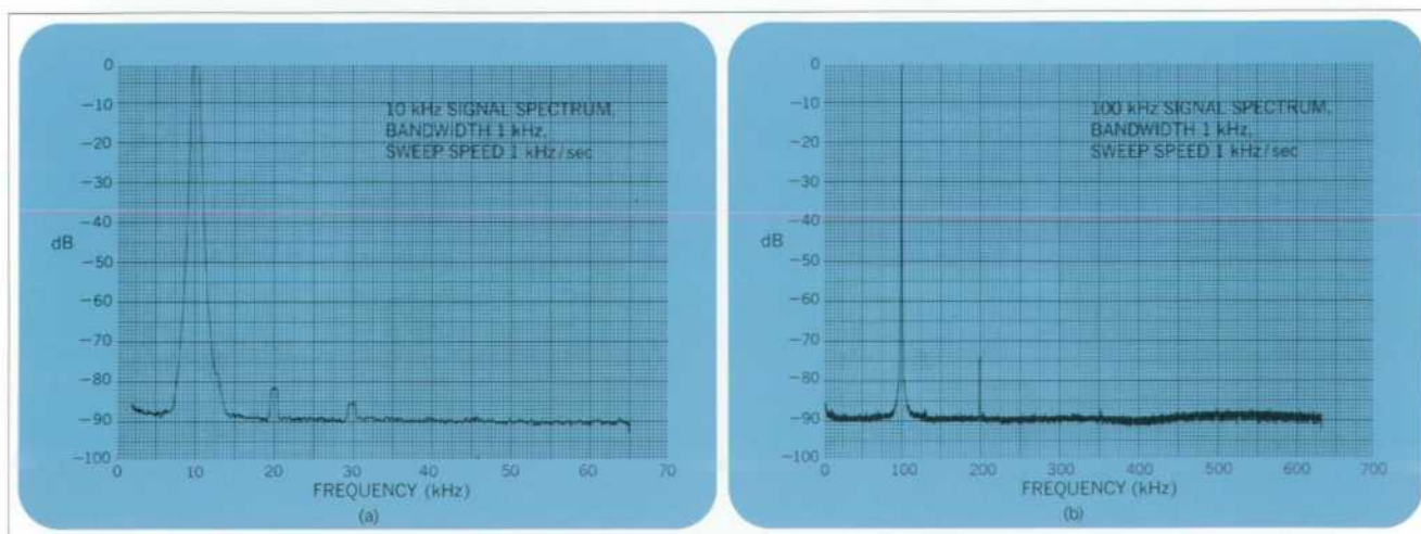
Fig. 6. Harmonic output of the Model 745A is better than 70 dB down, making it useful as a low-distortion oscillator, as well as a high-purity calibration standard.
