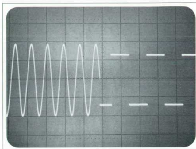
Fig. 5. Input waveform to the thermocouple. The sine wave is the instrument output, and the 500 Hz square wave is the reference. When there is an rms difference between these two, the thermocouple output is a 2 Hz square wave whose peak-to-peak value is proportional to this difference.
