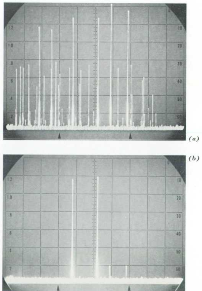
Fig. 4. (a) Without preselection, spectrum-analyzer display for strong (about 0 dBm) input signals at 4.9 and 5.1 GHz is complicated by intermodulation products and multiple responses. (b) Model 8441A Preselector reduces multiple responses and distortion products.
