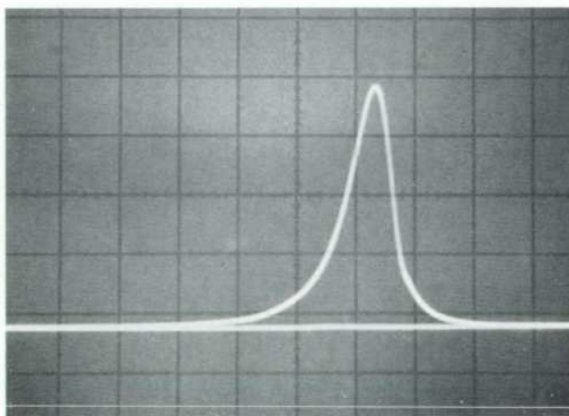
Fig. 6. Very low residual FM enables presentation of narrow sweep widths such as this crystal filter. This is a 20 kHz sweep width and the bandwidth of the filter is 1.5 kHz.
