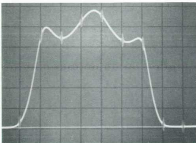
Fig. 5. Bandpass filter response from 11 to 21 MHz showing 1 MHz comb markers positioned exactly on each vertical line of the graticule.
