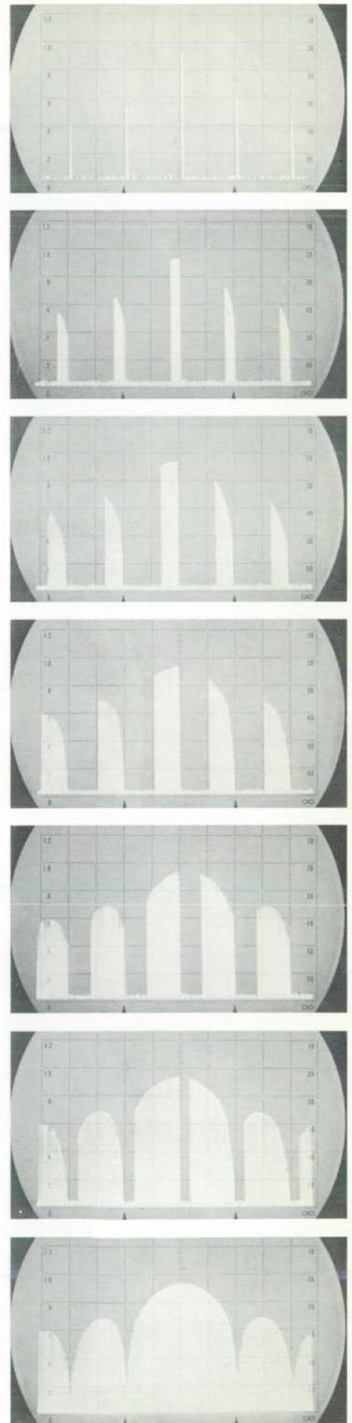
Fig. 7. Spectrum of a CW signal pulse-modulated at 50 Hz. Envelope of spectrum would be poorly defined with normal persistence, but gradually becomes well defined with variable persistence of new HP Model 852A Spectrum Analyzer Display Unit.
