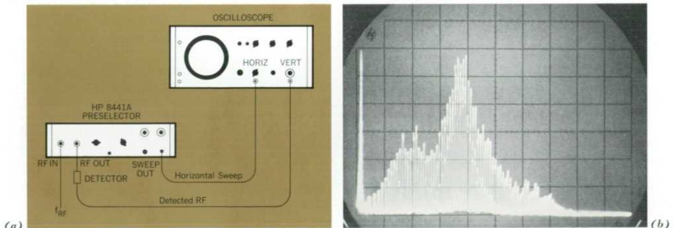
Fig. 6. (a) HP Model 8441A Preselector, with detector and oscilloscope, forms a low-sensitivity but very wideband spectrum analyzer. (b) Spectrum of high-power frequency comb obtained with spectrum analyzer setup (a). Sweep limits are 2 and 12 GHz.
