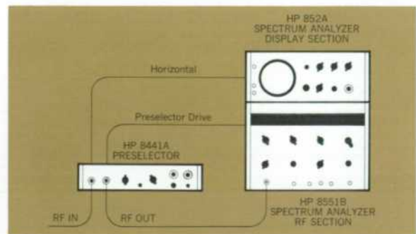
Fig. 2. New HP Model 8441A Preselector, connected to spectrum analyzer as shown, confines displayed signals to a selected frequency range. The preselector is a narrow-band YIG filter which automatically tracks a selected harmonic mixing mode of the analyzer's LO and mixer.
