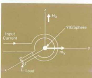
(f) Tuned bandpass filter consists of YIG sphere at center of two mutually orthogonal loops.
