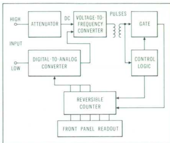
Fig. 4. Simplified block diagram of Model 3460A Digital Voltmeter. Control logic carries out sequence of operations automatically during each measurement interval.
