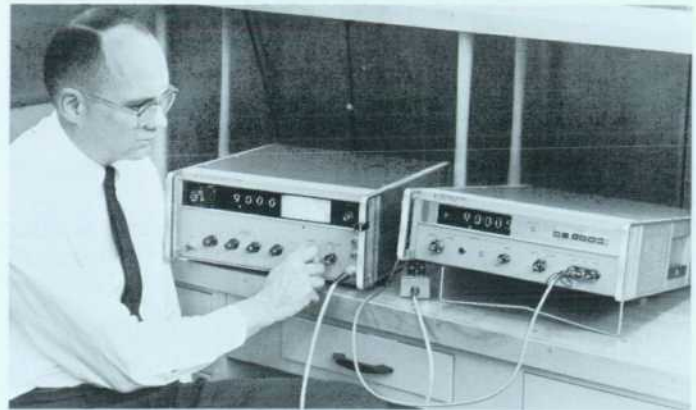
Fig. 1. New -hp- Model 3460A Digital Voltmeter, designed for either bench service or systems use, achieves standards lab accuracy with operating simplicity. Guarding preserves accuracy by eliminating effects of common-mode signals and instrument also has noise rejection properties of signal integration. As shown here, 0.005% accuracy of new digital voltmeter is such that it tracks output of dc voltage standard digit by digit.
