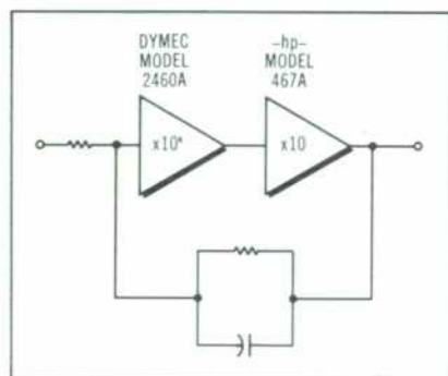
Fig. 11. Use of cascaded high-gain operational amplifier and new power amplifier achieves operational power amplifier of high stability.
