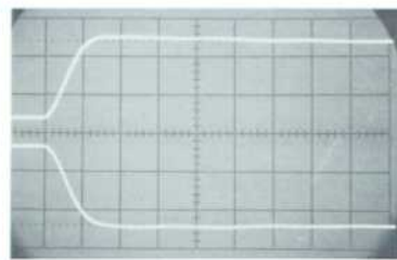
Fig. 4. Oscillogram shows typical step response of new Power Amplifier driving 40-ohm load for both positive and negative 1-volt steps at input. Sweep speed: 0.1 \mu\text{s}/\text{cm} ; vertical sensitivity: 5 V/cm.
