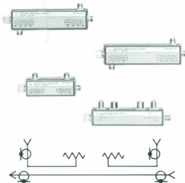
Fig. 10. Family of new -hp- Dual Directional Couplers and schematic diagram (below). From top to bottom, they are: Models 774D (215-450 Mc), 775D (450-940 Mc), 776D (940-1900 Mc) and 777D (1900-4000 Mc).
