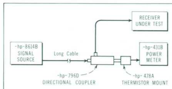
Fig. 5. Receiver sensitivity measurements uses -hp- Model 796D Directional Coupler to attenuate RF power 20 db below level indicated by power meter connected to main output.
