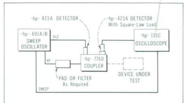
Fig. 9. Reflectometer system using hp - Model 776D Dual Directional Coupler. Forward auxiliary arm monitors RF level and supplies feedback signal to level sweep generator. Reverse auxiliary arm monitors reflected RF and supplies vertical signal for scope. Scope is calibrated for SWR by use of zero (short) or infinite (open) impedance loads (for details, see hp - Application Note 61).
