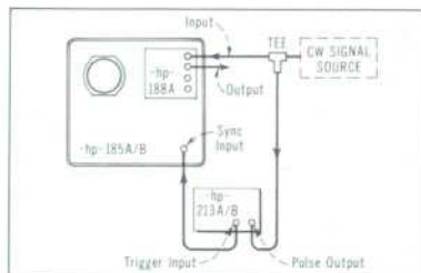
Fig. 12. Arrangement for using -hp- Model 213A/B, reverse-connected as shown, to trigger from signals to 4 Gc.
