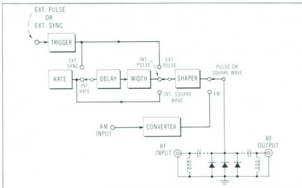
Fig. 5. Basic circuit arrangement of hp Model 8714A Modulator. Modulating mechanism is an array of p-i-n diodes acting as an electrically-controlled microwave attenuator.
