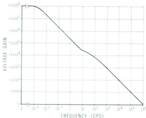
Fig. 8 (at right). Typical open-loop gain-band width characteristic of DY-2460A Amplifier.
