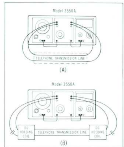
Fig. 6. Test set connections to telephone lines when dc is not present (a) and is present (b).
