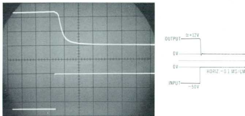
Fig. 4. Oscillograms showing typical fast recovery of new amplifier from large input overloads of 50 volts (a 500\times overload in \times 100 gain position).
