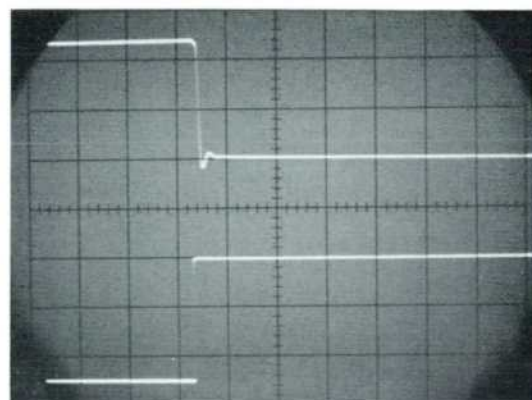
Left oscillogram is for \times 100 gain position using M2 plug-in, right for \times 10 position. Sweep time is 0.1 millisecond/cm (explanatory drawing in middle).
