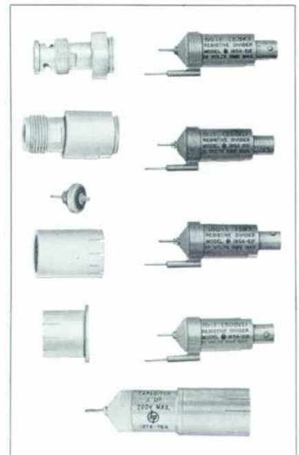
Fig. 5. A number of adapters and accessories permit connecting to fast waveforms with minimum circuit disturbance.
