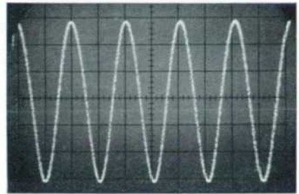
Fig. 4. Oscillogram of 1 kilomegacycle signal indicates stability of Model 185B synchronizing.
