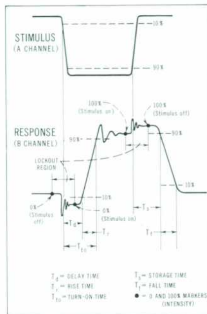
Fig. 6. Typical transistor measurements performed by dy-5844C System.
