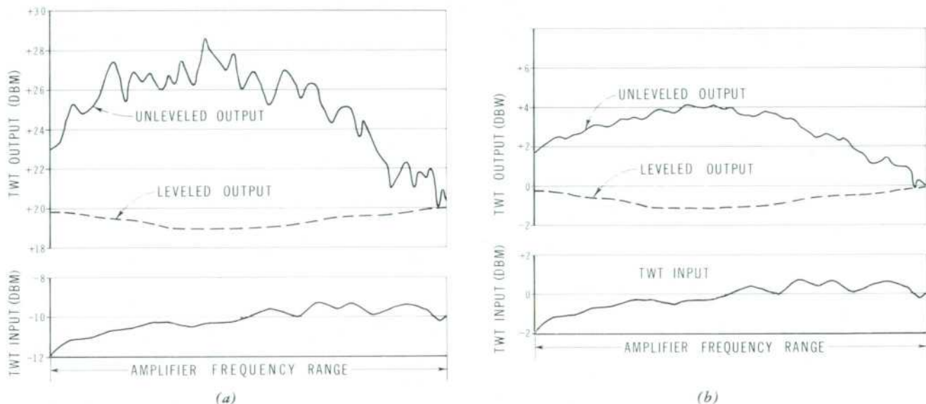
Fig. 5. Comparison of power output curves using new amplifiers at two input levels and in unlevelled and levelled applications.
