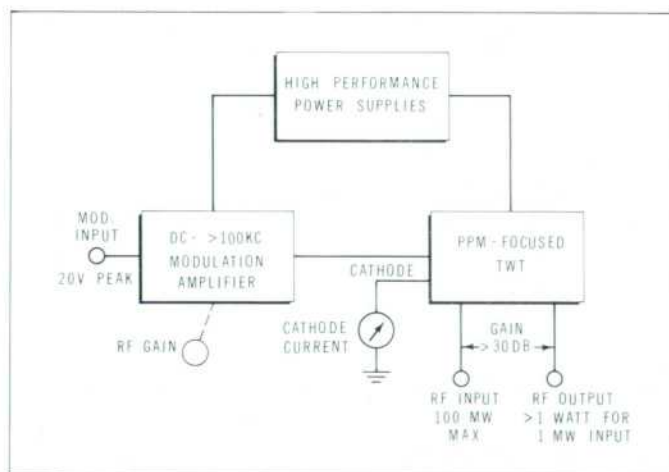
Fig. 2. Basic circuit arrangement of new amplifier units. Twt's are of periodic permanent-magnet-focused type.
