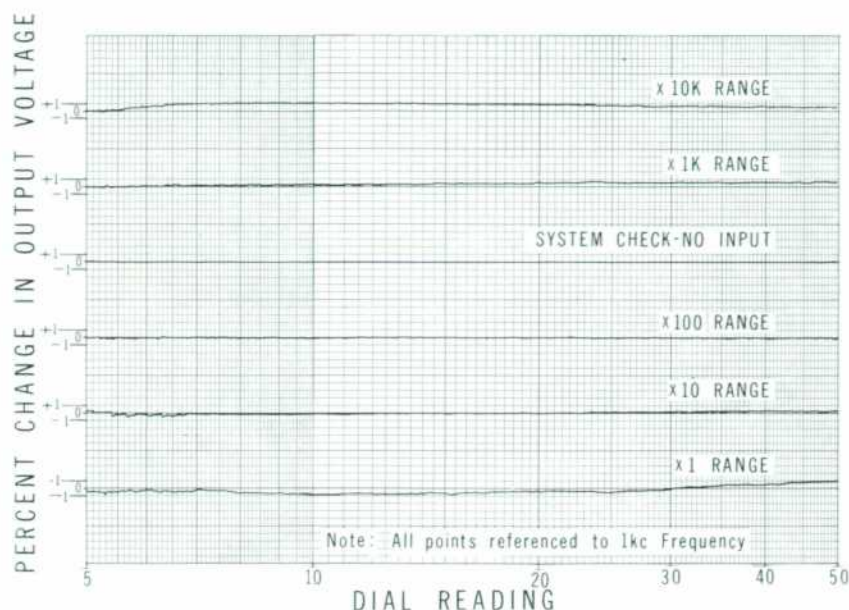
Fig. 5. Effectiveness of amplitude control circuit as shown by typical frequency response characteristic of Model 204B. Each minor vertical division has value of 1% so overall response is within about \pm 1\% .
