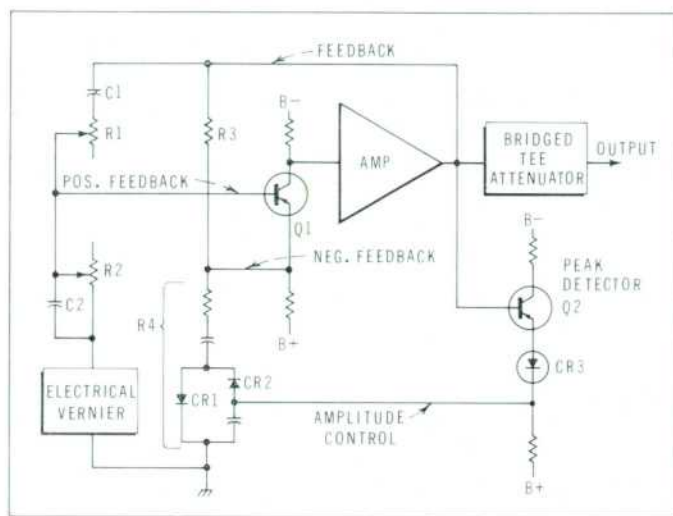
Fig. 3. Basic circuit arrangement of new RC oscillator. For power economy new amplitude control circuit replaces traditional ballast lamp, but frequency response is very constant as shown in Fig. 5.
