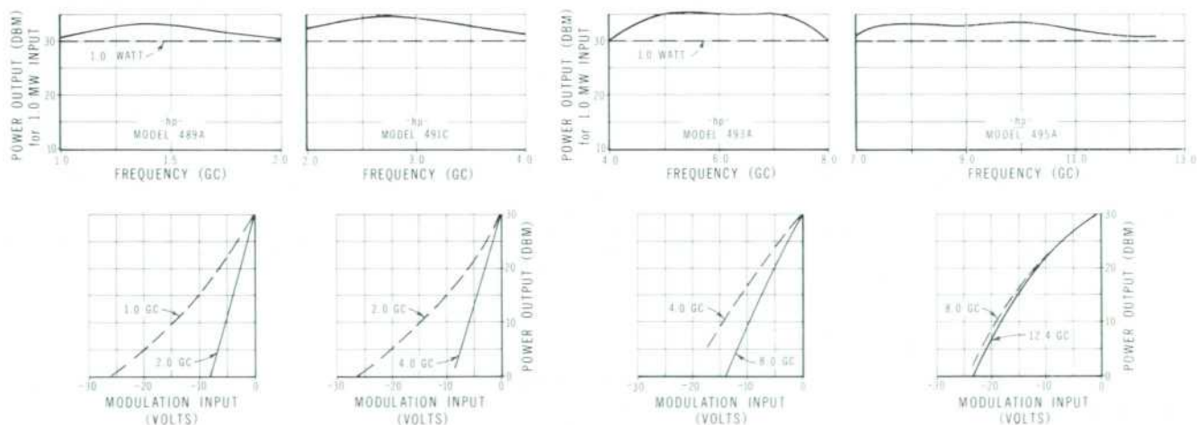
Fig. 6. Typical power output characteristics for new Microwave Amplifiers.
