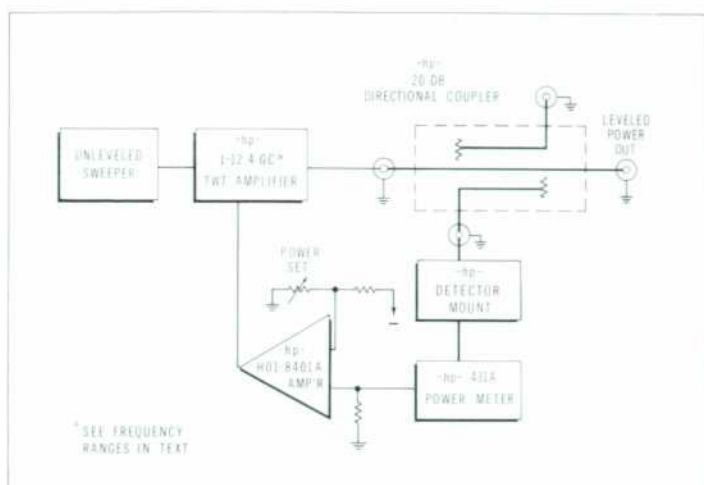
Fig. 4. Equipment arrangement for forming constant-power 1-watt sweepers using new amplifiers with unlevelled, low-power sweep generator.
