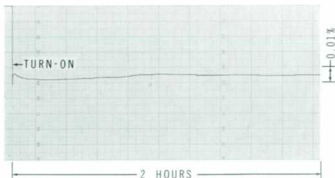
Fig. 2. Typical frequency-stability characteristic of Model 204B Oscillator. Frequency drift was only about 1 part in 20,000 in complete test including turn-on drift. Instrument begins to operate almost immediately after turn-on.
