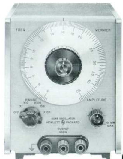
Fig. 4. hp Model 204B Transistorized Oscillator.
