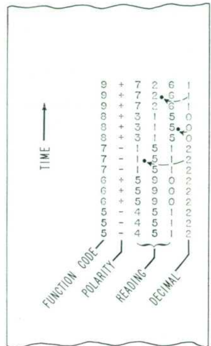
Fig. 4. Typical print-out obtained when voltmeter is used with hp digital recorder and operated with a programmer for multi-point measurements. First column identifies measured test point, while remaining columns indicate measured voltage.
