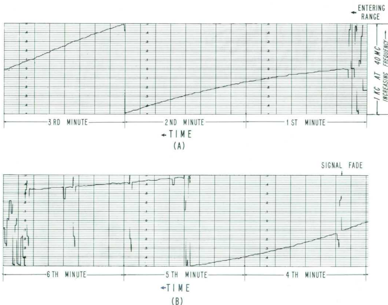
Fig. 1. Record of doppler shift in 40-megacycle transmission from Russian earth satellite made by Stanford Research Institute, Menlo Park, California.
