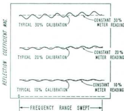
Fig. 6. By suitably adjusting gain control on Model 416A Ratio Meter, response of measurement system can be recorded before measuring device under test to facilitate reading of record. Response can be recorded at various levels as shown or at any convenient value. See text.
