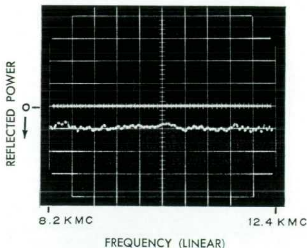
Fig. 8. Typical oscilloscope display obtained when calibrating setup of Fig. 7 using internal square-wave modulation on the sweep oscillator.
