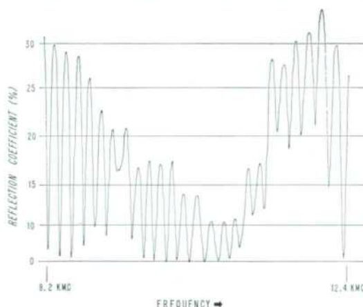
Fig. 2. Permanent record of output reflection coefficient of TWT indicates how such records can be used to provide product performance data and to insure freedom from unknown peaks or holes.
