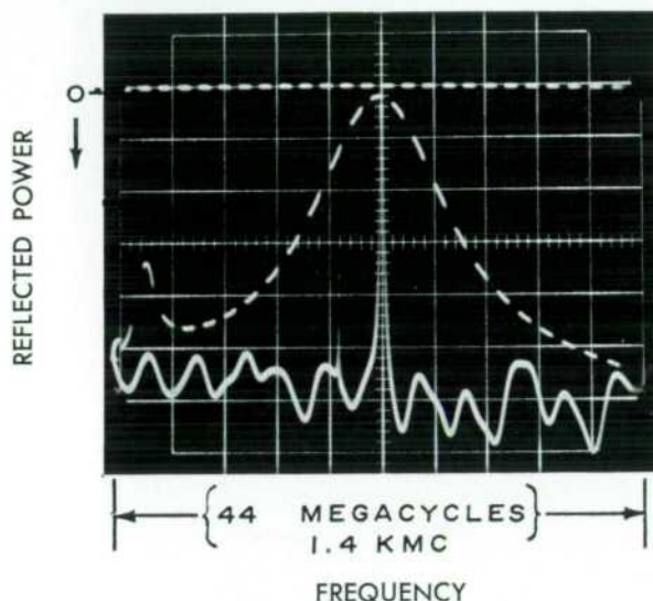
Fig. 11. Double exposure oscillogram of resonance characteristic of reflex klystron at two r-f sweep widths. Dashed (square wave modulated) trace has 32 times narrower range than solid trace. Wave meter pip at extreme left of dashed trace has been moved from its position in solid trace so that it is about \frac{1}{2} down skirt of resonance curve, accounting for its apparent lower level in dashed trace.
