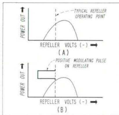
Fig. 4. (a) Typical power output vs. repeller voltage characteristic of klystron used in -bp- microwave generators. (b) Positive modulating pulse applied to repeller circuit klystron out of oscillation.
