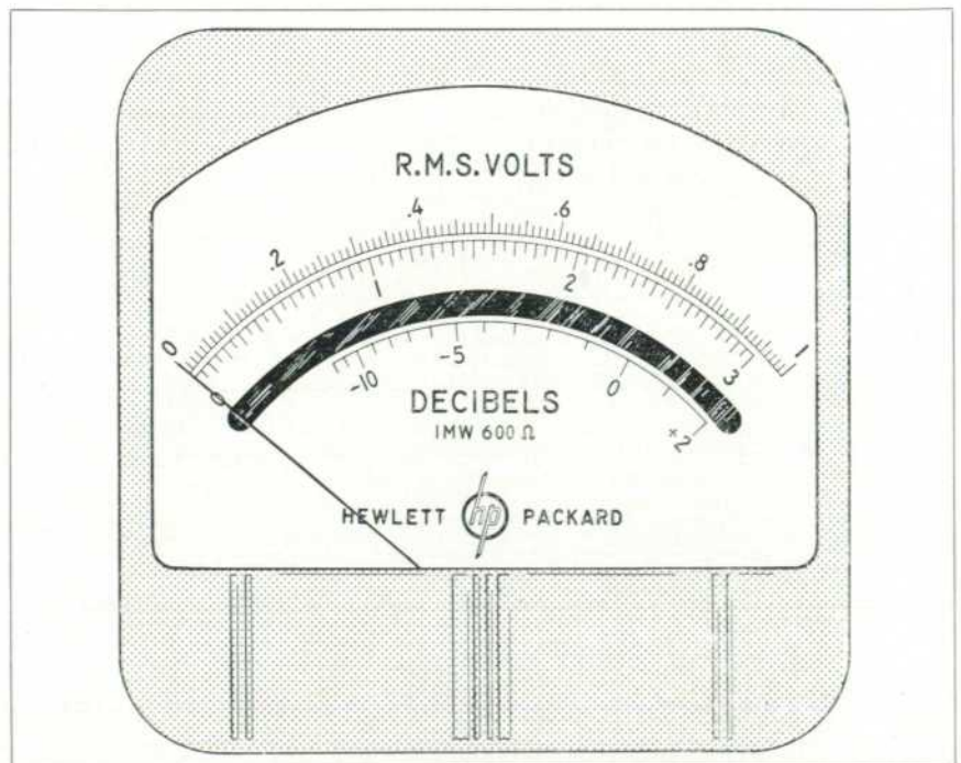
Fig. 4. Two-thirds size reproduction of meter used in Model 400H. Upper scale is calibrated in 1% increments, "3" scale in 1.7% increments.
