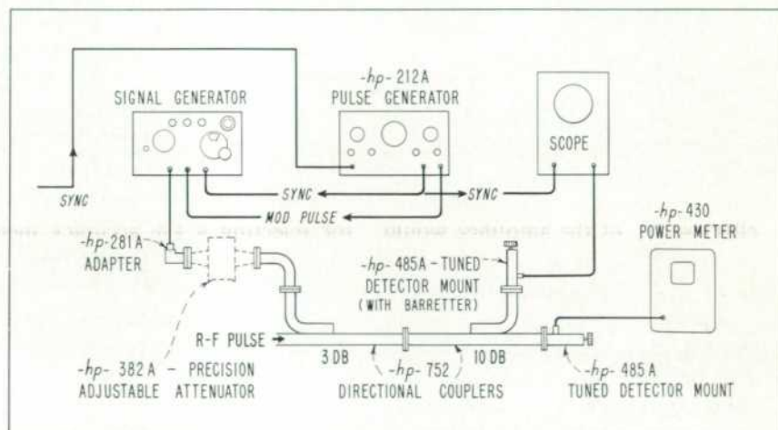
Fig. 2. Typical equipment arrangement for forming notch wattmeter at X-band frequencies.
