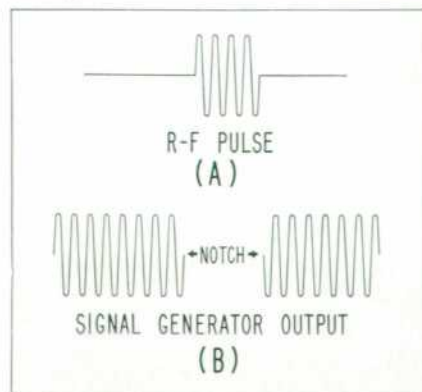
Fig. 1. Sketch illustrating (a) typical r-f pulse to be measured; (b) pulse-off type output required from signal generator.
