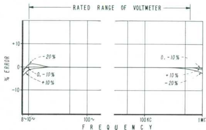
Fig. 3. Typical effect of +10 to -20% G_m variations in tubes in Model 400AB.
