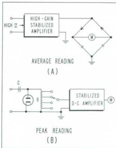
Fig. 1. (a) Average-reading type circuit used in -hp- 400 series voltmeters to obtain relative freedom from waveform effects as discussed in accompanying article. (b) Peak-reading type circuit used in -hp- 410 voltmeters. Although this circuit has greater sensitivity to waveform effects, it is possible, through suitable design to operate the circuit up to hundreds of megacycles as in the -hp- 410B 700-megacycle voltmeter.
