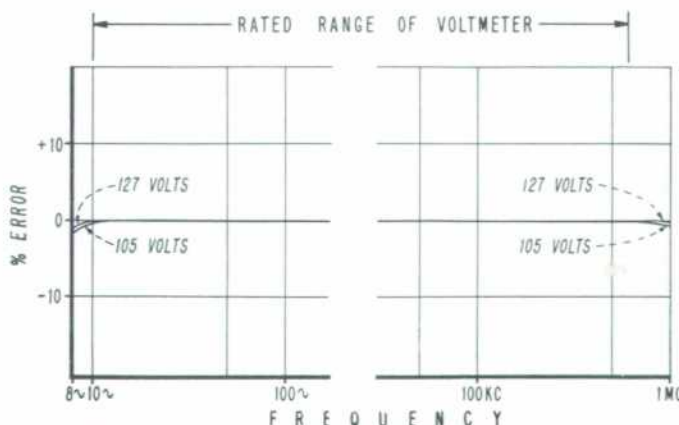
Fig. 2. Typical accuracy of Model 400AB. Effect of line voltage changes from 105 to 127 volts is perceptible only at extremes of range.
