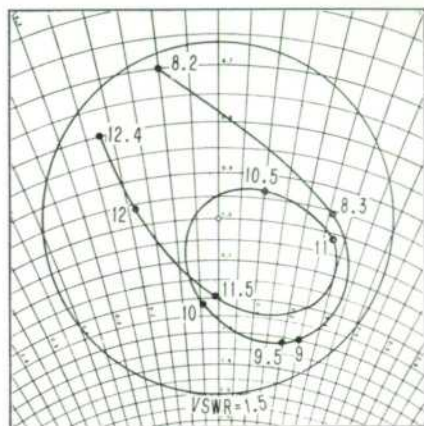
Fig. 4. Typical impedance characteristic of waveguide thermistor mount for 8.2 to 12.4 kmc range (Model X487A).
