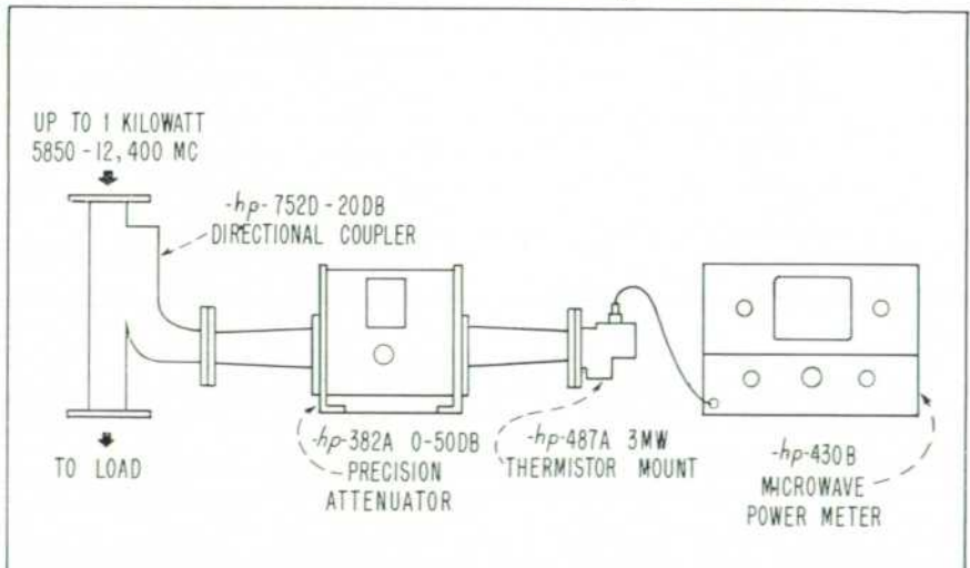
Arrangement for monitoring average powers up to 1 kilowatt in waveguide systems. -hp- Model 750D series cross-guide directional couplers may be used in place of Model 752D. See note above concerning attenuator. For monitoring coaxial systems, -hp- 281A series coax-waveguide transitions can be used at each end of directional coupler.
