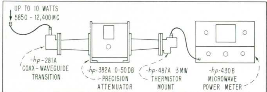
Arrangement for measuring average powers up to 10 watts in coaxial systems. -hp- Model 370 series fixed attenuators, rated at 1 watt, may be useful in some applications in place of 10-watt Model 382A adjustable attenuator.
