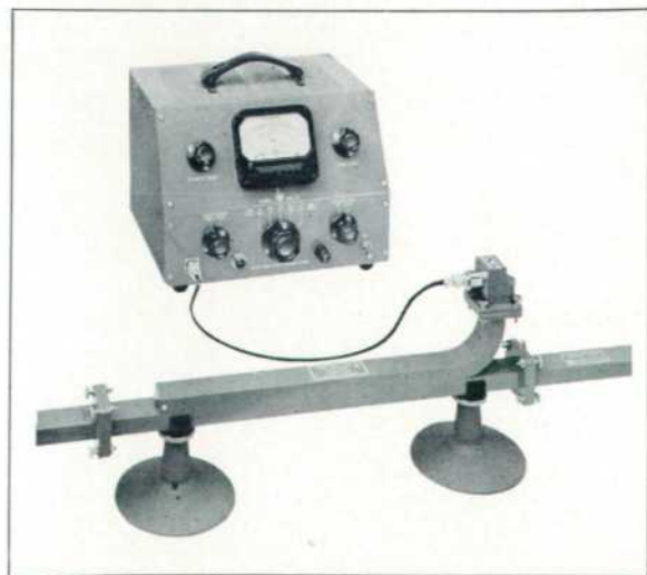
Fig. 1. New -hp- Model 487A broadband thermistor mount used with directional coupler and power meter to monitor power level in waveguide system.
