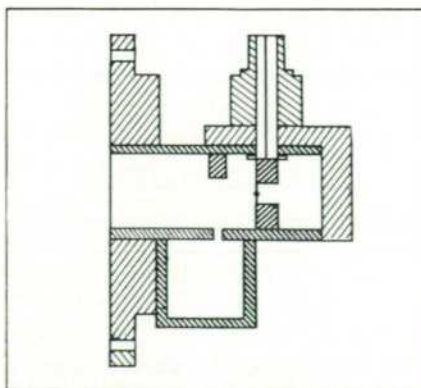
Fig. 3. Simplified cross-sectional drawing of Model 487A waveguide mount.
