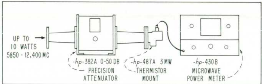
Arrangement for measuring average powers up to 10 watts in waveguide systems. See note above concerning attenuators.
