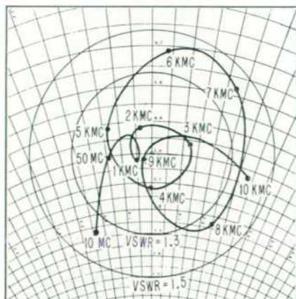
Fig. 6. Typical admittance characteristic of -bp- Model 477A coaxial thermistor mount.
