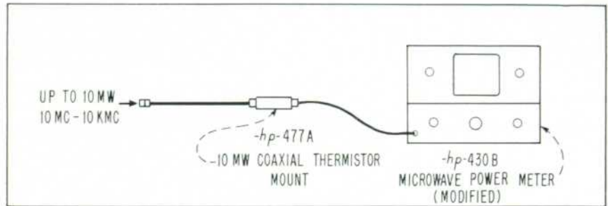
Arrangement for measuring average powers up to 10 milliwatts in coaxial systems.
