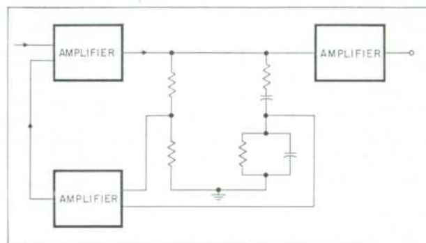
Fig. 3. Basic arrangement of selective amplifier in -hp-206A.
