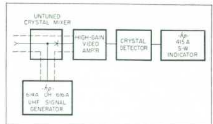
Fig. 4. Simple laboratory receiver using hp Model 614A or 616A as local oscillator.
