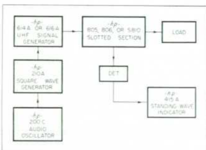
Fig. 3. Typical set-up for standing-wave measurements using hp Model 614A or 616A. Use of high-gain Model 415A Standard Wave Indicator increases sensitivity of measurements.
