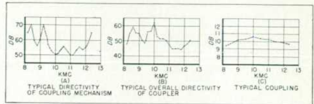
Fig. 5. Characteristics of typical -hp- 10 db multi-hole coupler.
