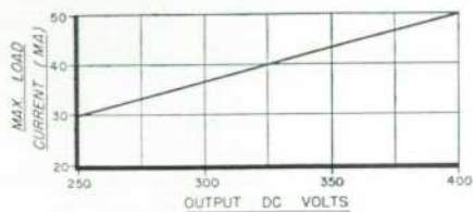
Figure 2. Current de-rating curve for -hp- Model 715A.
