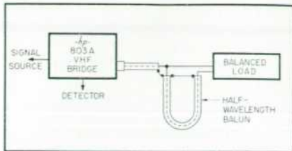
Figure 1. Measurement set-up using balun with balanced load.
