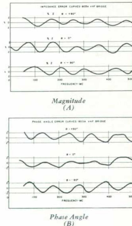
Figure 5. Typical Correction Curves Supplied with Bridge.
