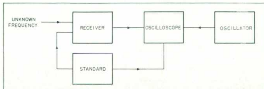
Figure 5. Set-up for Measuring High Frequencies.
