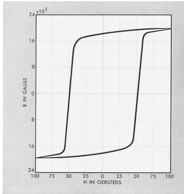
A typical do hysteresis loop of Remendur composition developed for the series ferreed. The square-ness ratio is 0.9. Illustrating the isotropic qualities of the alloy, this loop was measured at 90 degrees to the rolling direction of the processed strip.
