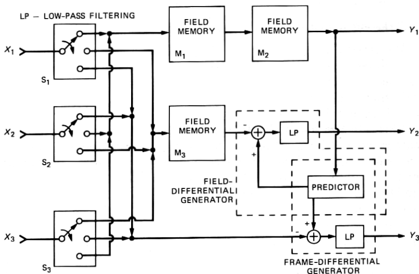
Fig. 2—The differential-signal multiplexer.
