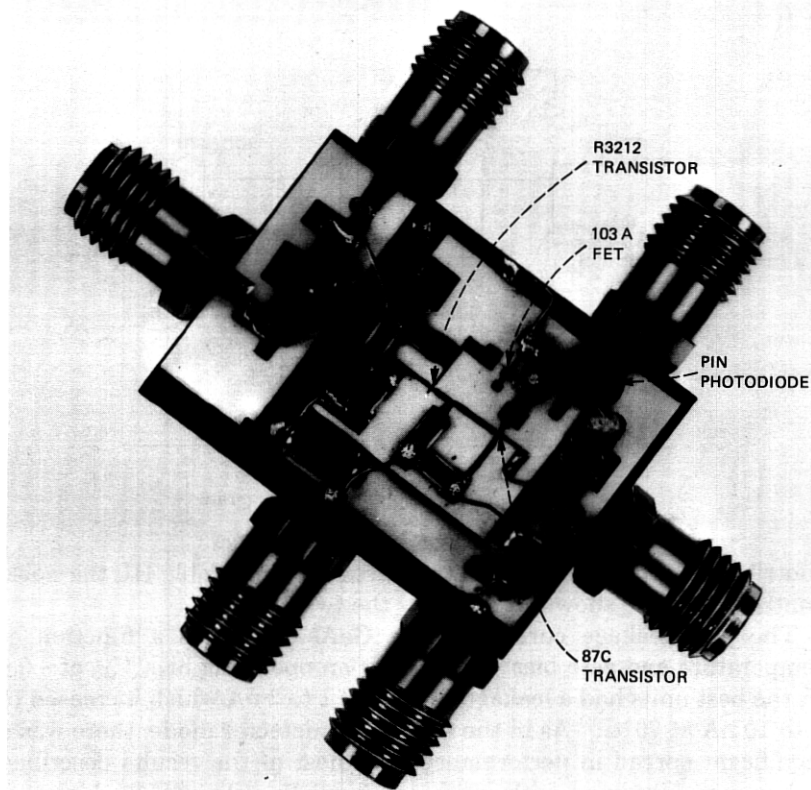
Fig. 10—Front-end module with coaxial test connections.
