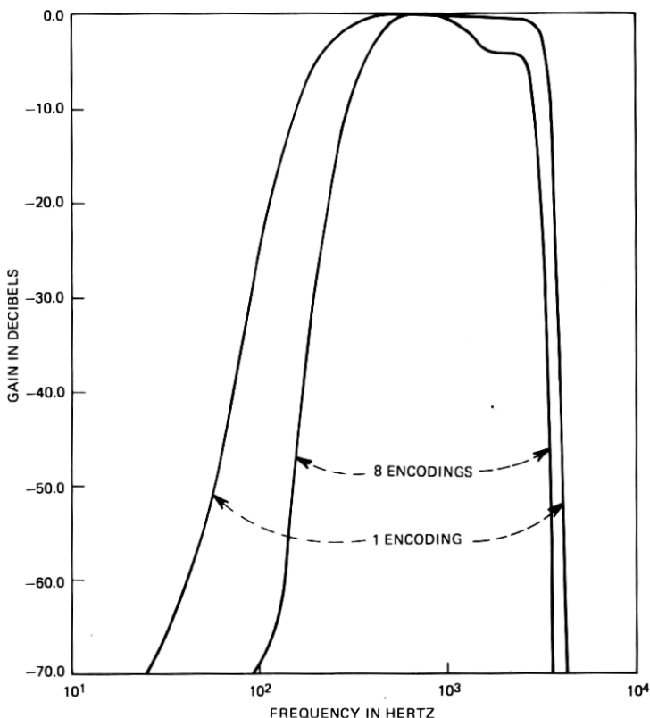
Fig. 13—Overall frequency response—37.7 kHz—one and eight encodings.
