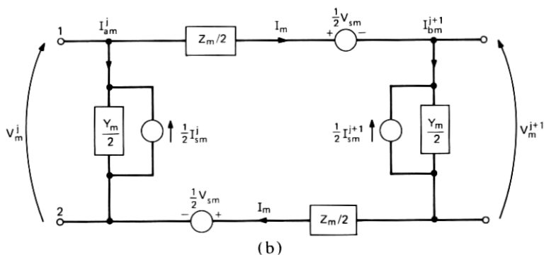
Fig. 6—Longitudinal-to-metallic conversion model. (a) Segment of a longitudinal circuit. (b) Segment of a metallic circuit.
