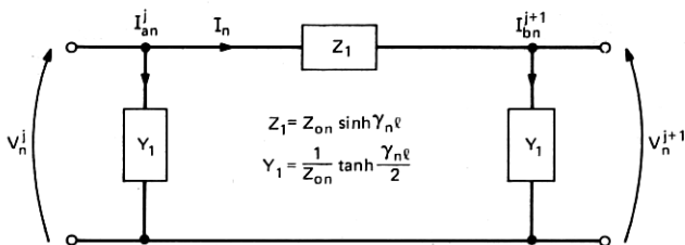
Fig. 8—Equivalent network for a general transmission line.
