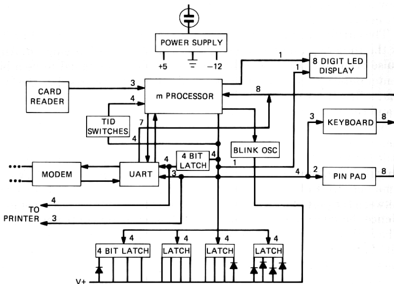
Fig. 6—Transaction III block diagram.
