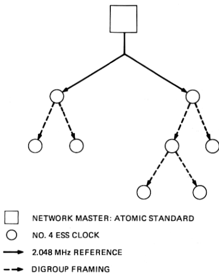
Fig. 9—Master-slave timing structure.
