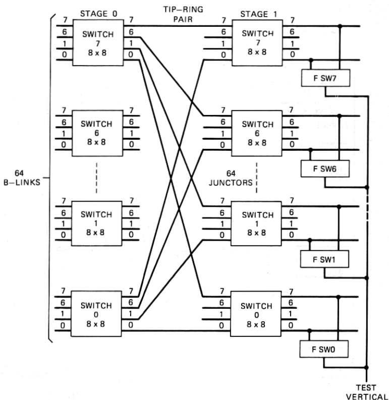
Fig. 7—Junctor-switching frame—tip-ring block diagram of a grid with test-vertical access.
