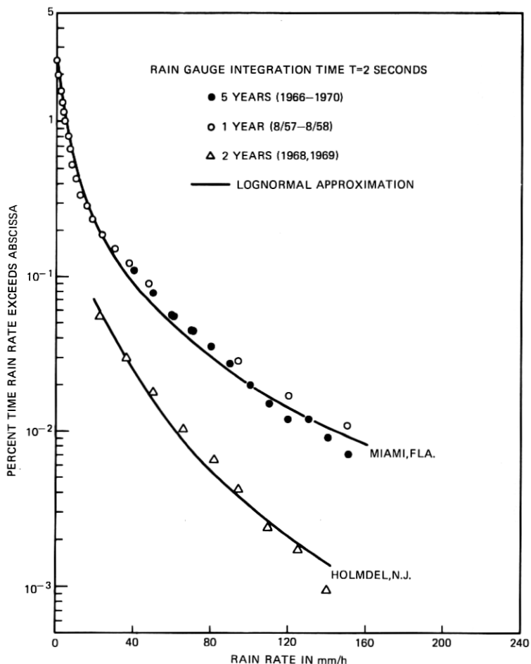
Fig. 11—Lognormal distribution of 2-s point rain rate at Miami, Florida and Holmdel, New Jersey.
