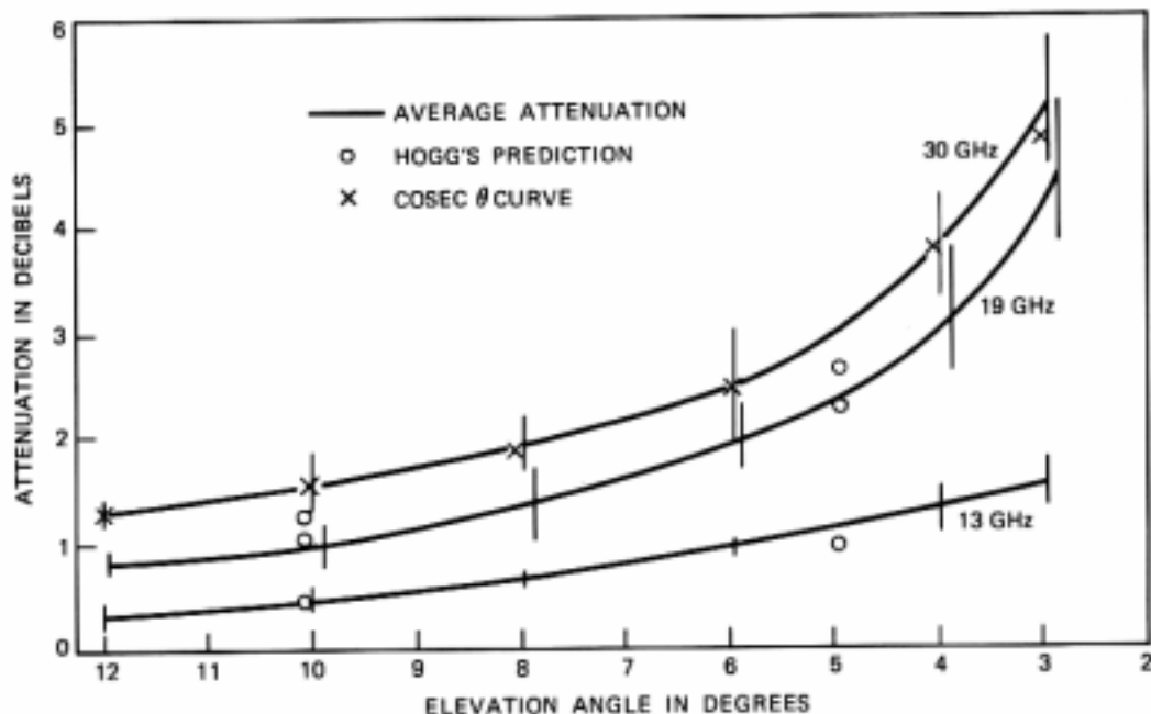
FIG. 1—Attenuation vs elevation angle, normal summer weather (average humidity 12.5 gm/m 3 ).
