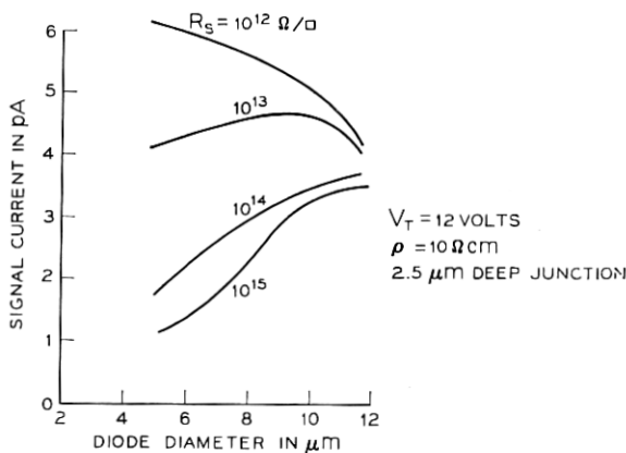
Fig. 20—Single diode signal capability for Q_{ss}/q = 3 \times 10^{11} \text{ cm}^{-2} .
