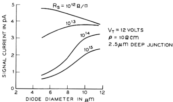
Fig. 18—Single diode signal capability for Q_{ss}/q = 1 \times 10^{11} \text{ cm}^{-2} .
