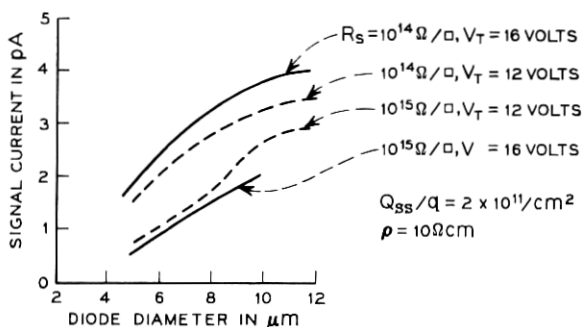
Fig. 22—Effect of bias on single diode signal capability.
