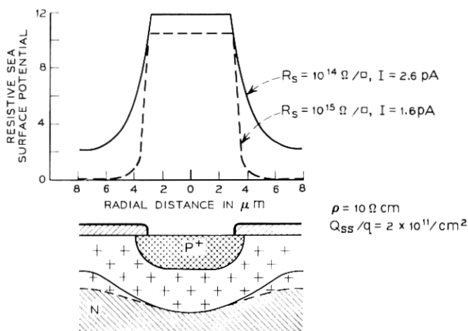
Fig. 16—Discharged conditions for 6 \mu\text{m} window diode.
