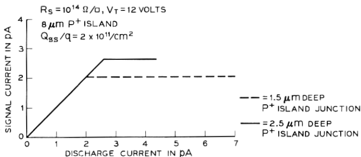
Fig. 21—Effect of P^+ island depth on single diode signal characteristic.
