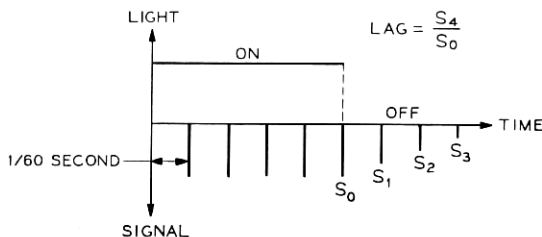
Fig. 25—Definition of lag.
