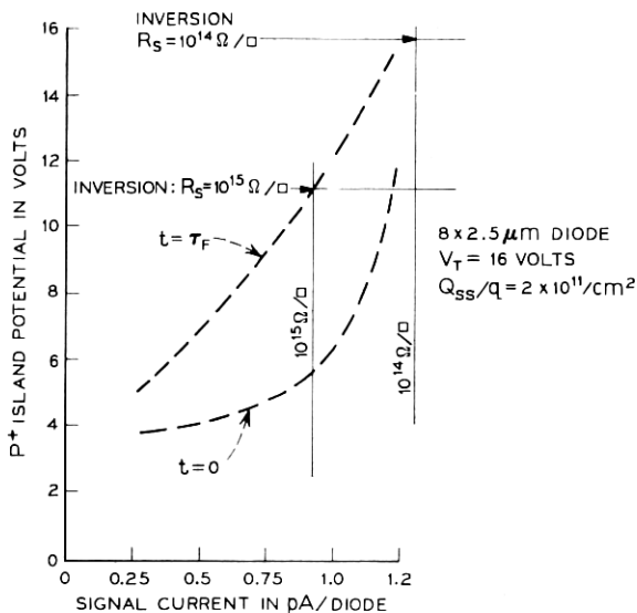
Fig. 24—Calculated P + island potential extremes as a function of discharge current.
