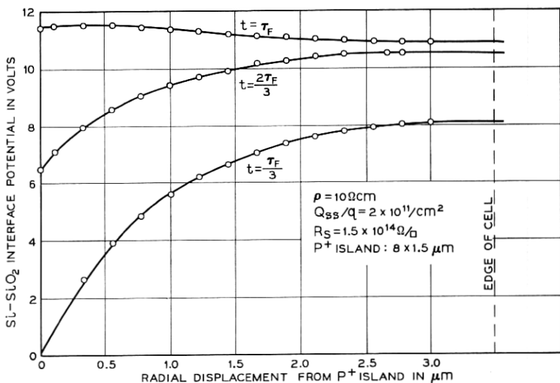
Fig. 12—Si-SiO 2 interface potential at the end of three equal time intervals during discharge.
