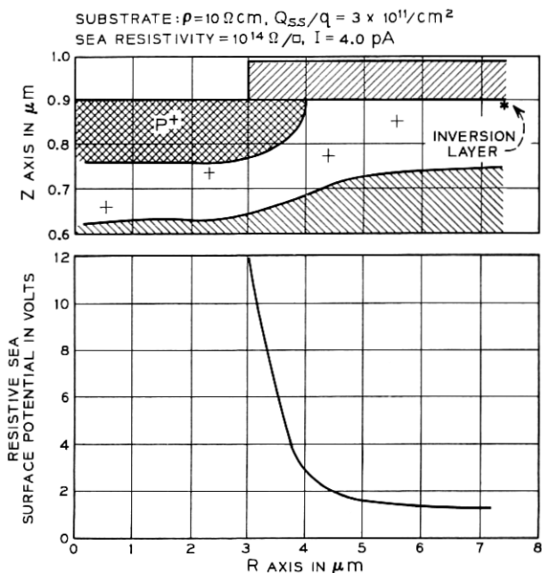
Fig. 11—Calculated discharged conditions for above total surface depletion operation.
