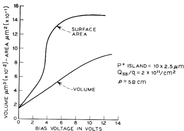
Fig. 28—Calculated depletion region geometric factors.
