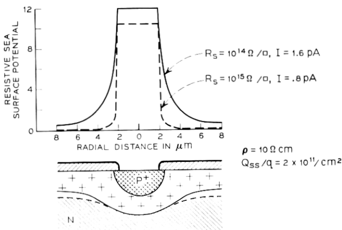
Fig. 15—Discharged conditions for 4 \mu\text{m} window diode.
