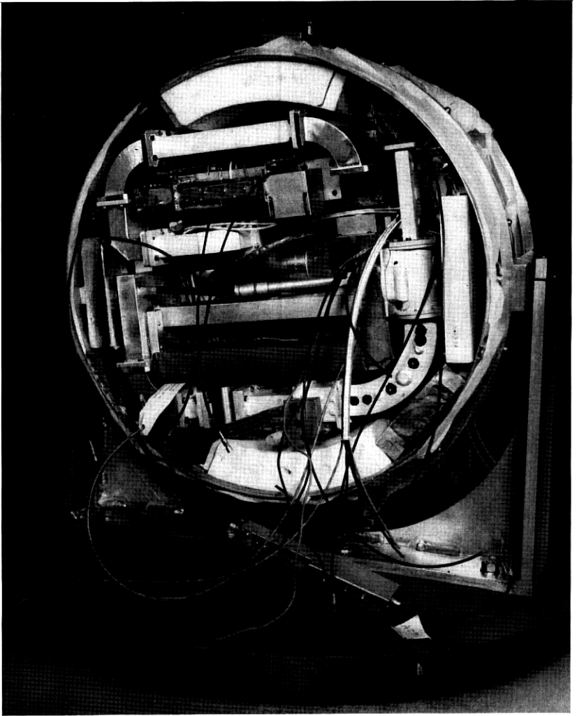
Fig. 7 — The electronics canister.
