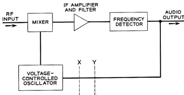
Fig. 1 — Simplified block diagram of FMFB system.
