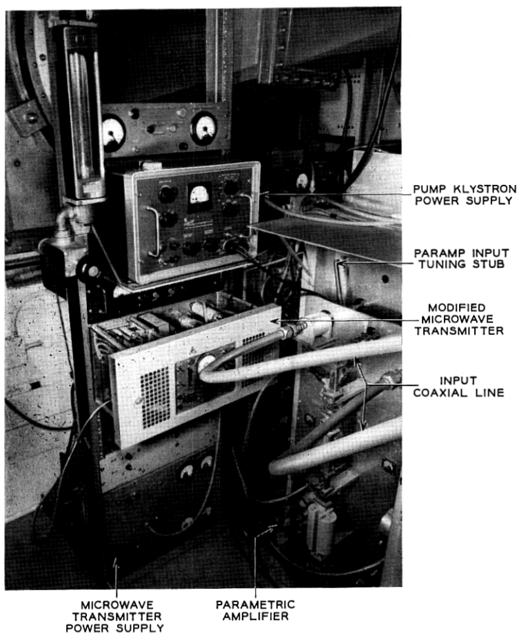
Fig. 12 — Parametric amplifier coaxial input lines, power supply mountings and microwave transmitter.
