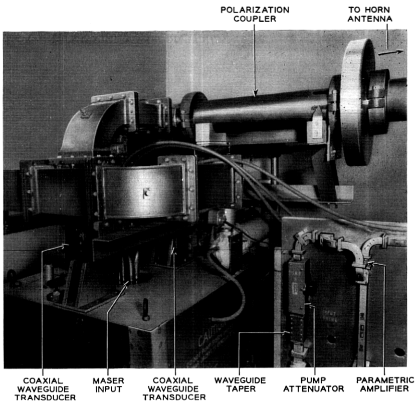
Fig. 10 — Position of parametric amplifiers and masers relative to the polarization coupler.
