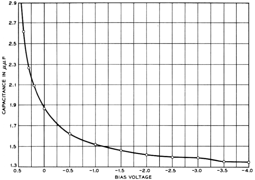
Fig. 3 — Capacitance vs. voltage for the silicon mesa varactor diode.
