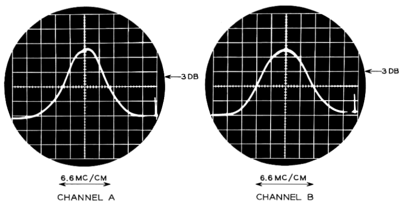
Fig. 6 — Parametric amplifier band-pass characteristic for channels A and B.
