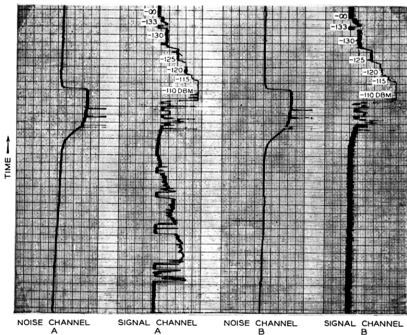
Fig. 14 — Recording of signal levels received by the parametric amplifier system from JPL, pass 93. Signal levels increase from left to right.
