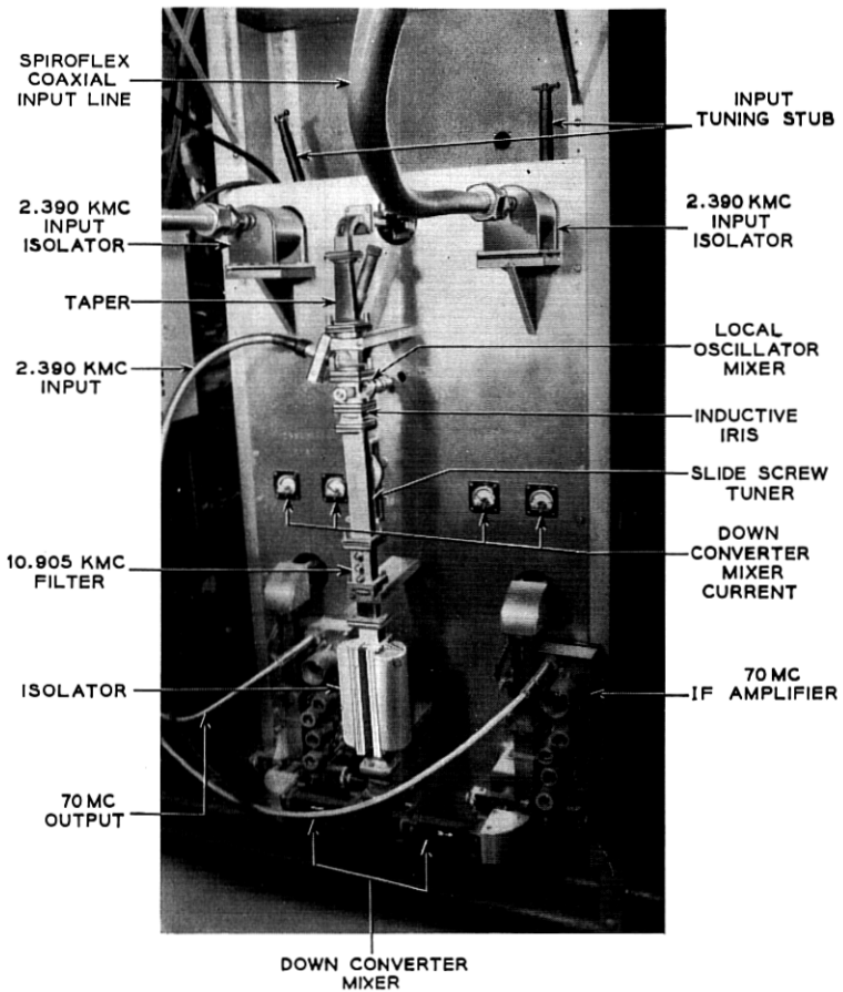
Fig. 8 — Dual parametric amplifiers mounted on support frame (side 2).
