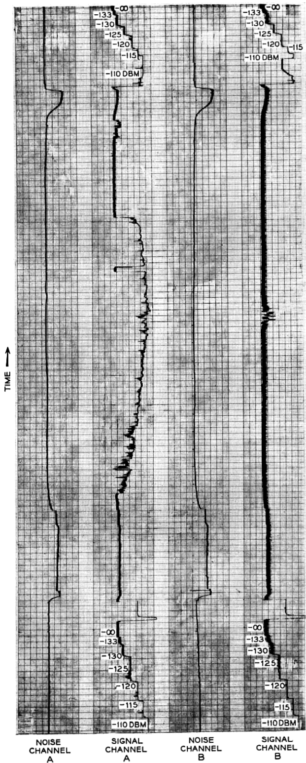
Fig. 15 — Recording of signal levels received by the parametric amplifier system from JPL, pass 94. Signal levels increase from left to right.
