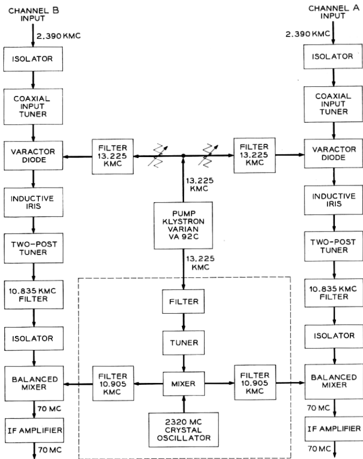
Fig. 2 — Block diagram of parametric amplifier system.
