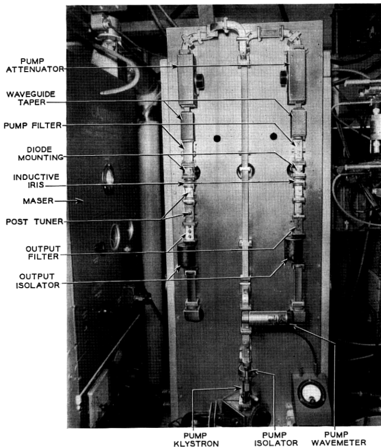
Fig. 7 — Dual parametric amplifiers mounted on support frame (side 1).
