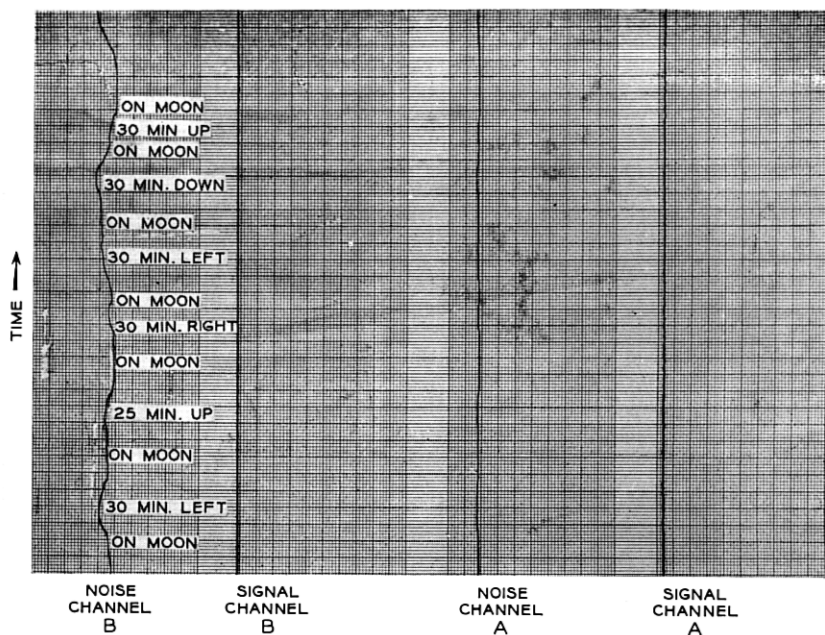
Fig. 13 — Noise signal received by the parametric amplifier system as the antenna scanned the moon.
