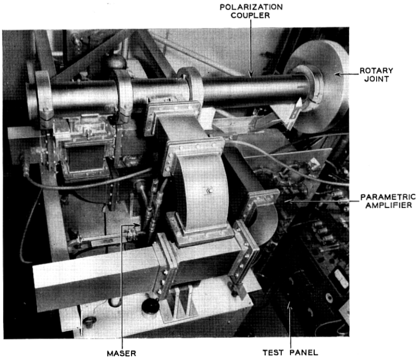
Fig. 9 — Relative position of parametric amplifier and maser in antenna cab.
