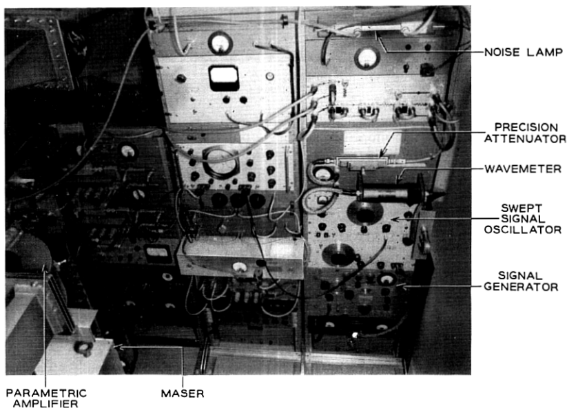
Fig. 11 — Test panel in the antenna cab.
