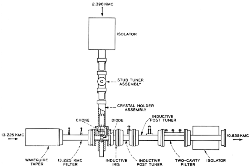
Fig. 5 — Assembly diagram of a single parametric amplifier.
