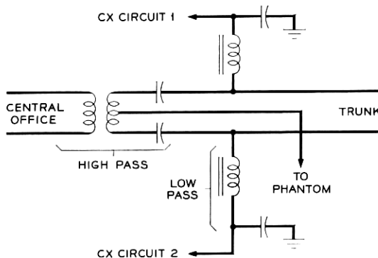
Fig. 7 — CX circuit for one end of a trunk pair.
