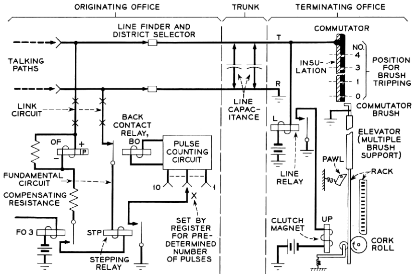
Fig. 11 — Retractive pulsing between panel offices.
