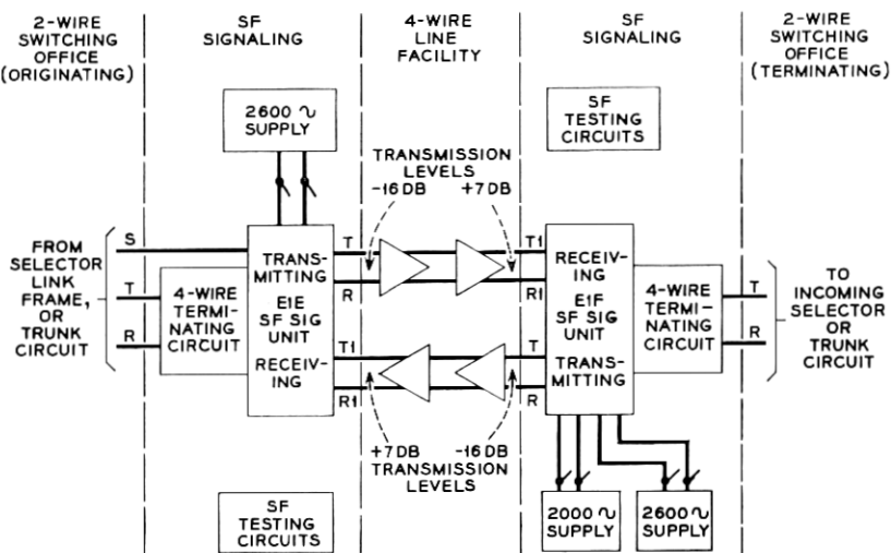
Fig. 19 — Circuit layout using SF signaling unit for revertive pulsing.
