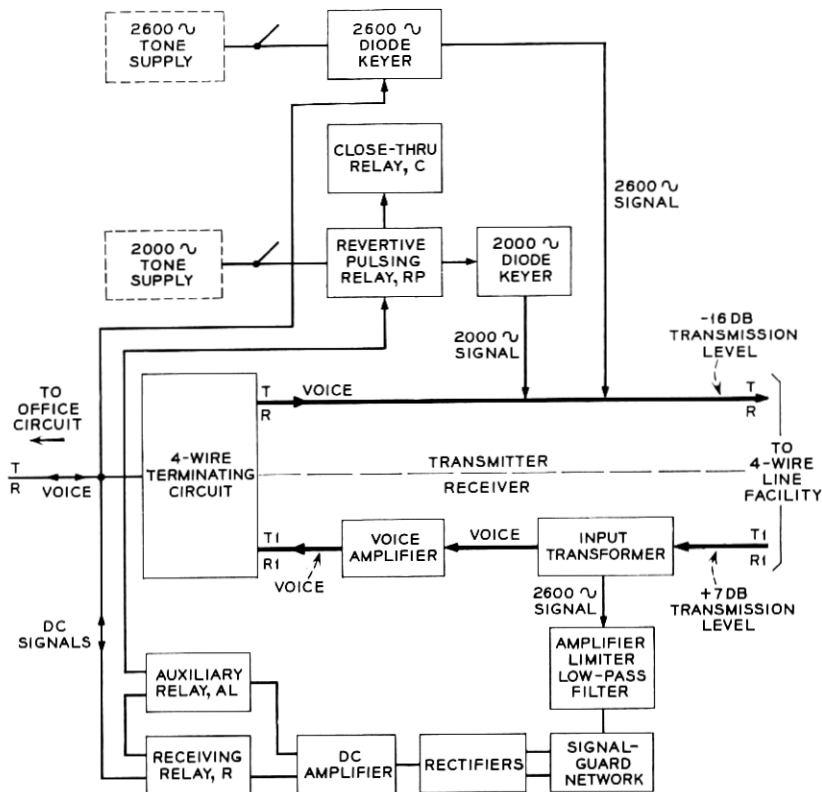
Fig. 21 — Basic elements of SF signaling unit — terminating terminal reverberative pulsing.
