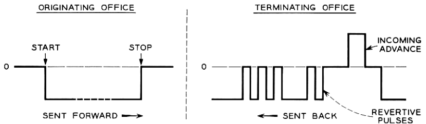
Fig. 12 — Retractive pulsing.
