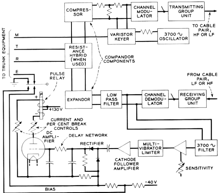
Fig. 18 — N-1 carrier signaling system (out-of-band).
