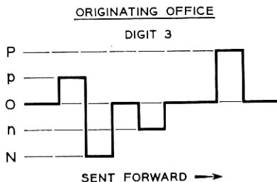
Fig. 13 — PCI pulsing.
