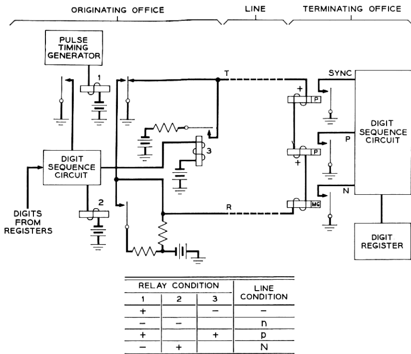
Fig. 14 — Basic PCI pulsing system.
