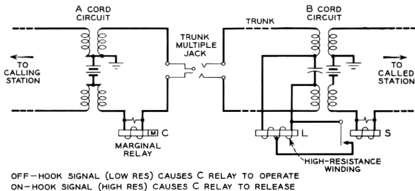
Fig. 2 — High-low signaling.
