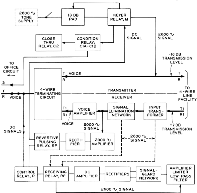
Fig. 20 — Basic elements of SF signaling unit — originating terminal reverive pulsing.
