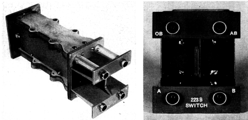
Fig. 6 — 223-type IF coaxial switch.
