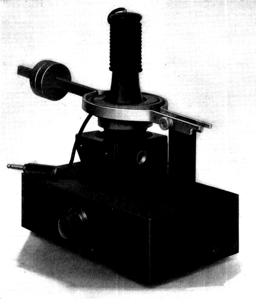
Fig. 12—Artificial ear coupler.
