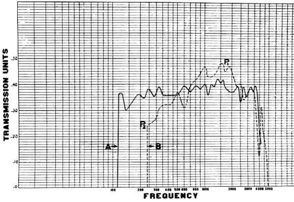
Fig. 20—Response frequency characteristic of two phonographs. Curve A shows the characteristic of the band pass filter type described. Curve B shows the characteristic of one of the best commercial machines previously on the market
