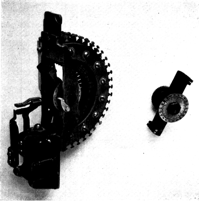
Fig. 19—Sender Selector
