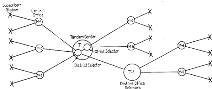
Fig. 27—Tandem Trunking Plan Showing Distant Office Selector
