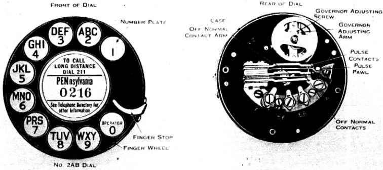
Fig. 6—Subscriber's Dial
